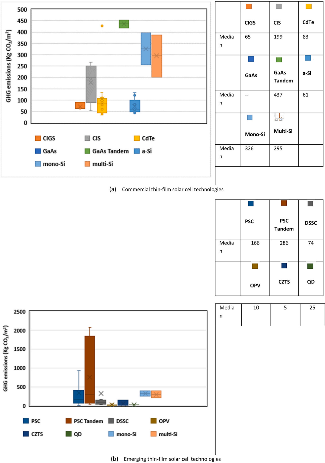
Fig. 6. Review of global warming potential (GWP) of various thin-film solar cell technologies in comparison to the conventional Si-based technologies.
