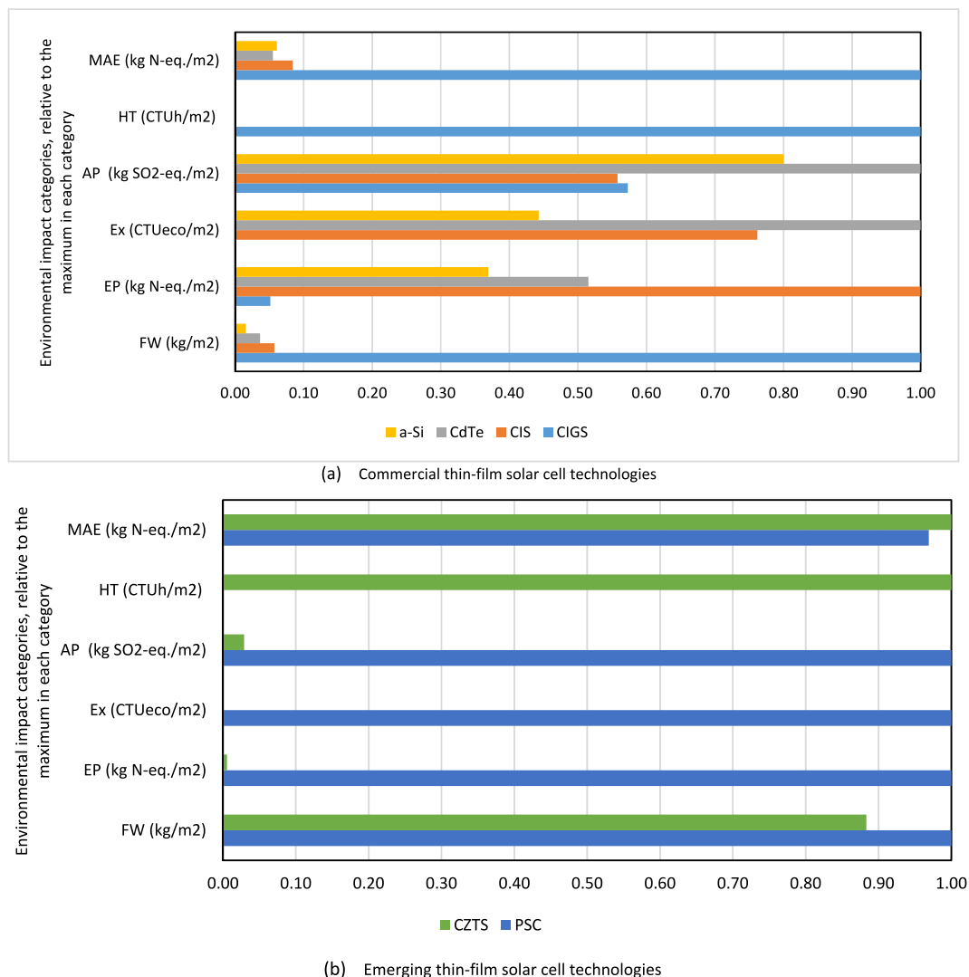
Fig. 7. Environmental impact of different thin-film solar cell technologies (Data are displayed relative to the maximum)
