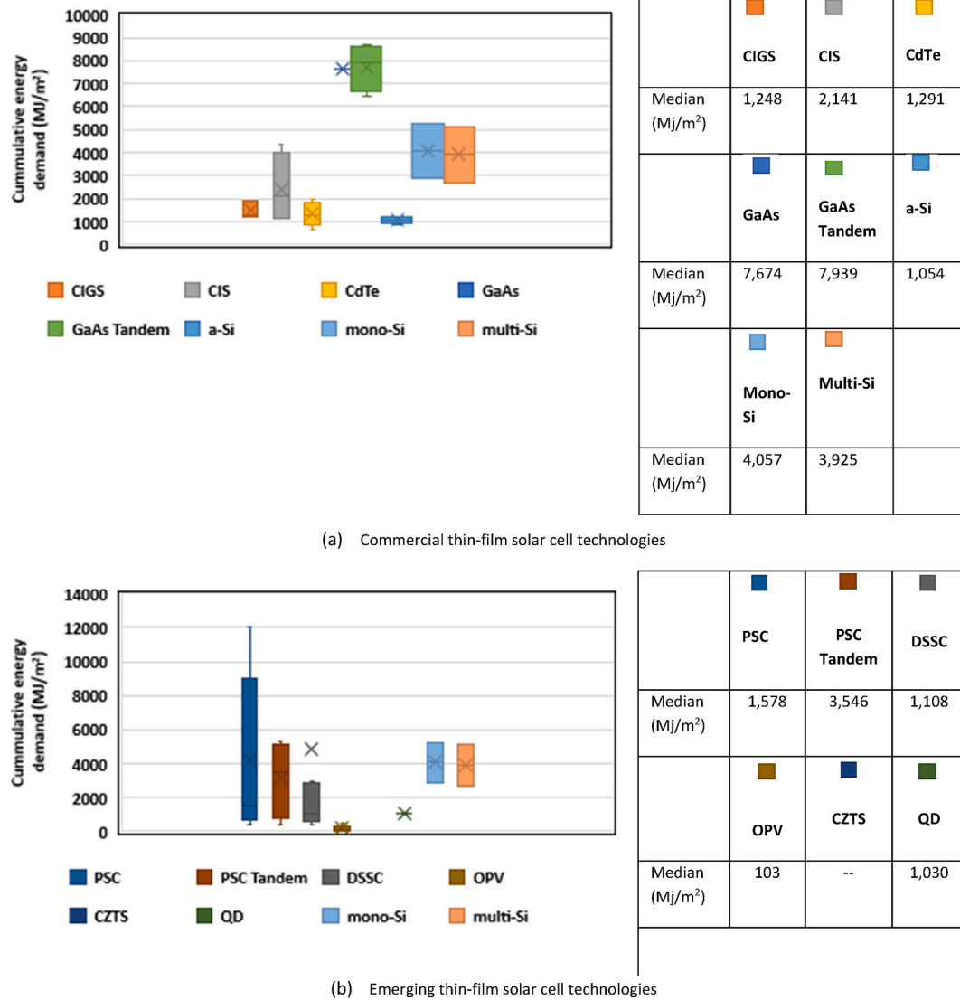
Fig. 5. Review of cumulative energy demand (CED) during the life cycle for various thin-film solar cell technologies in comparison to conventional Si-Based technologies.
